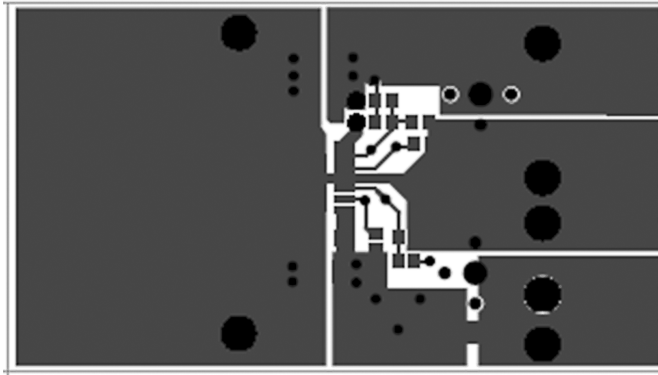
Figure 2. Top Layer
