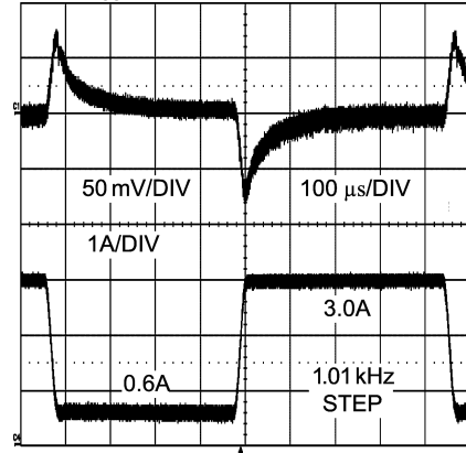
LMZ14203 Transient Response V_{IN} = 24V V_{OUT} = 3.3V , 0.6 A to 3A Step
