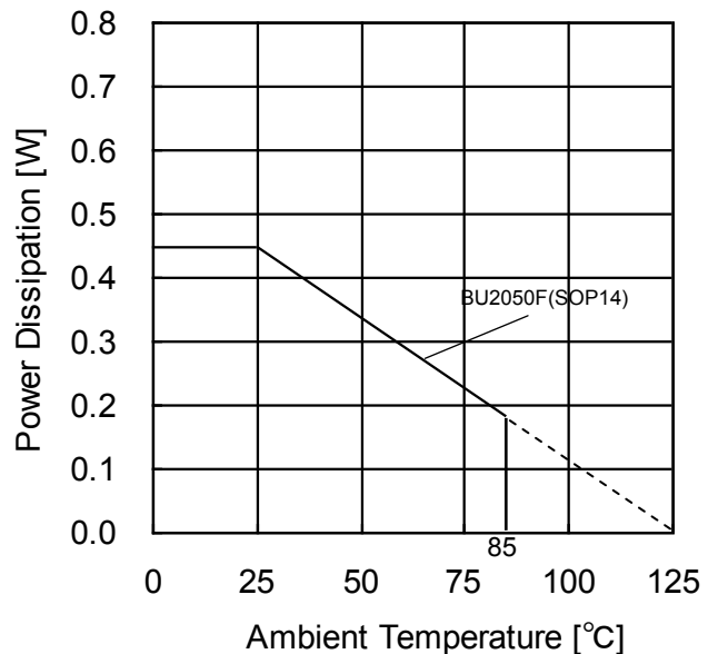
Figure 9. Derating Curve
