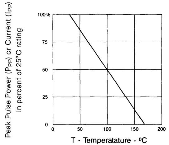
FIGURE 2 DERATING CURVE
