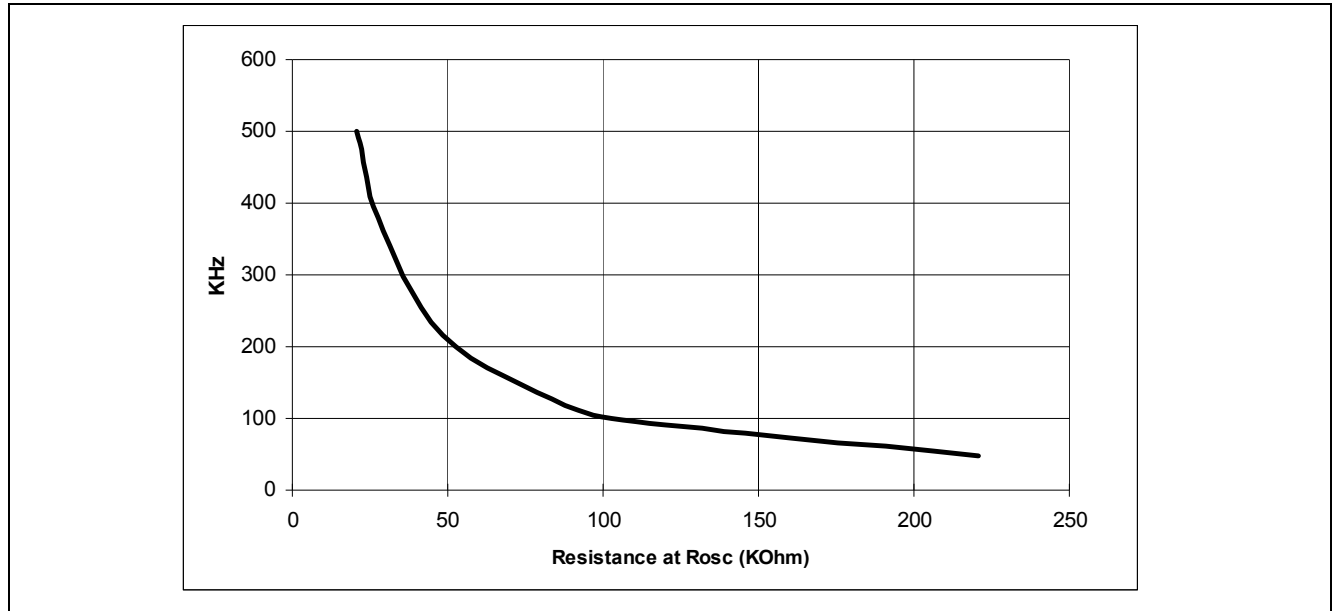
Figure 8 Internal Frequency Setting at R_{osc}
