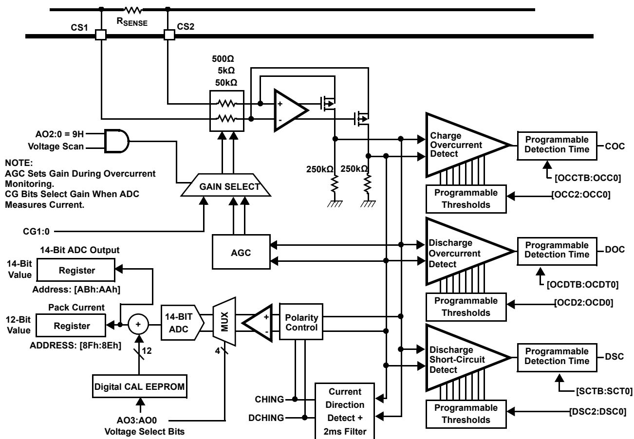
Figure 51. Current Sense
