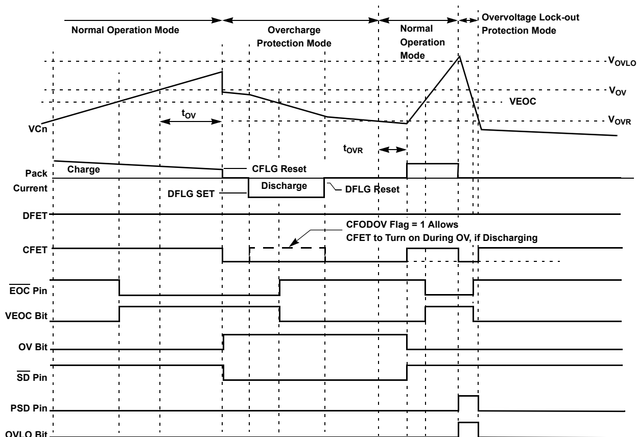
Figure 65. OV Detection/Response
