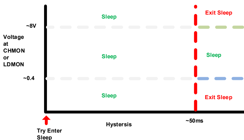
Figure 45. SLEEP Qualification
