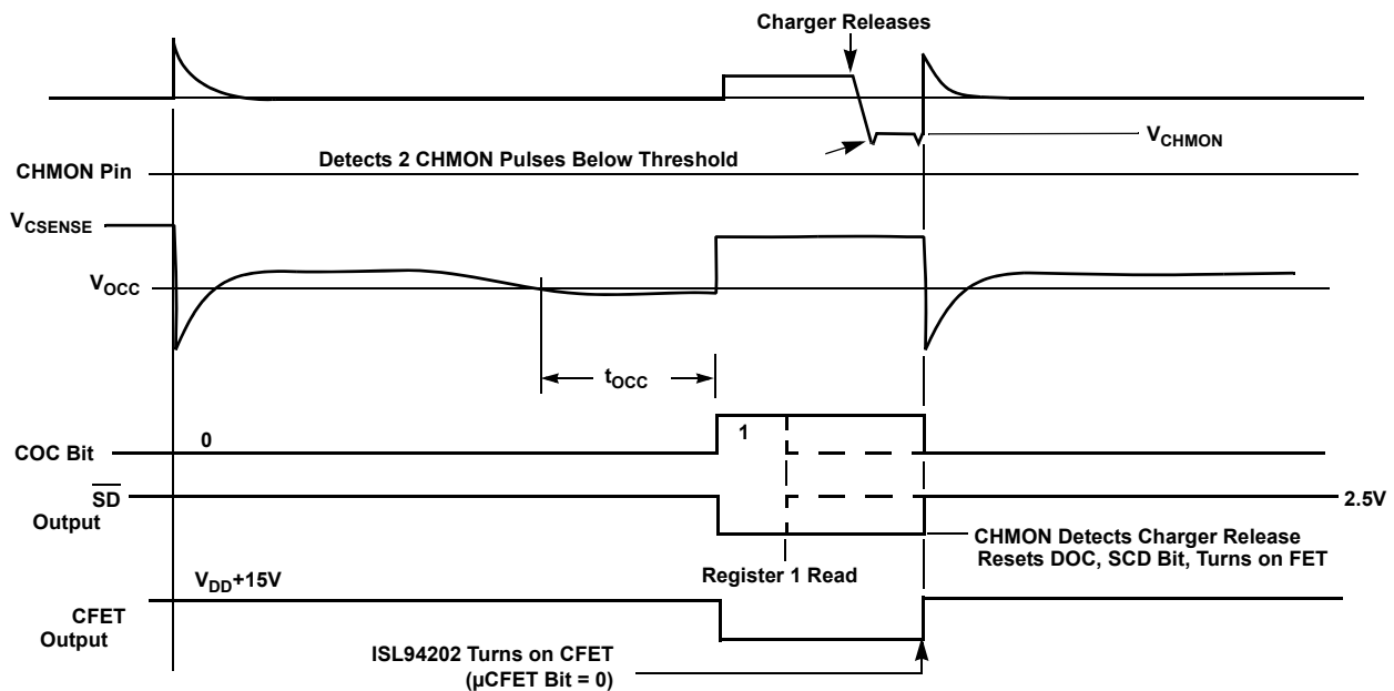
Figure 36. COC Recovery
