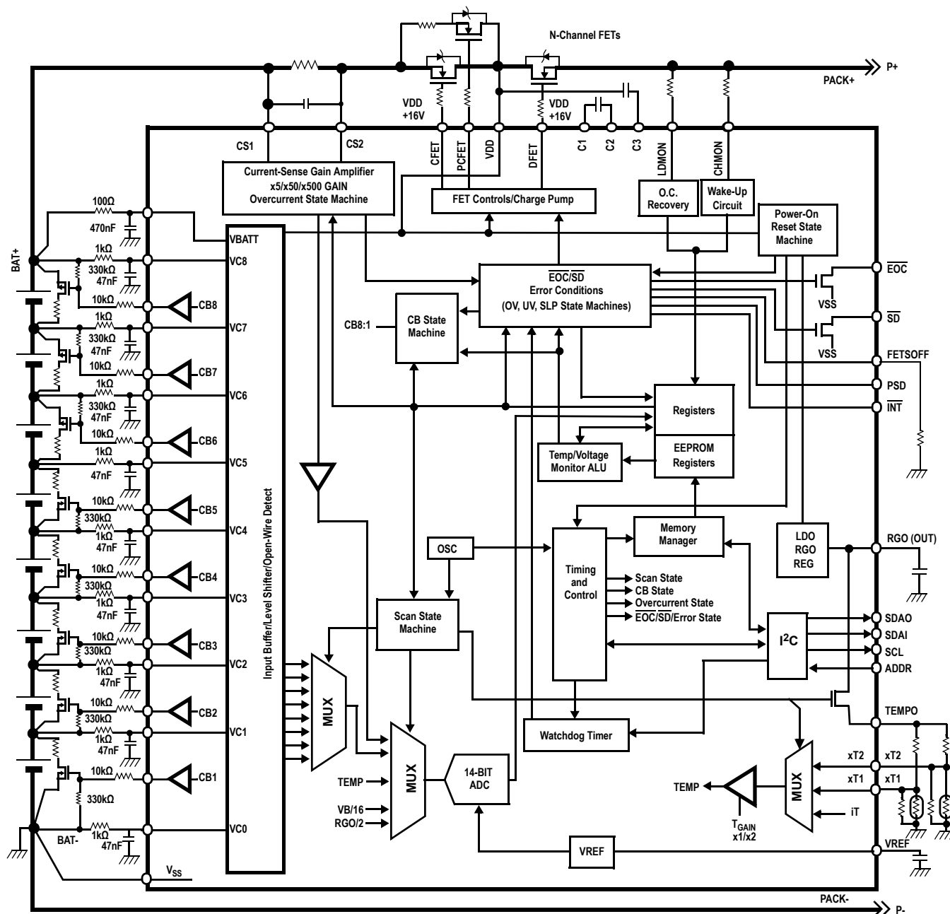
Figure 2. Block Diagram
