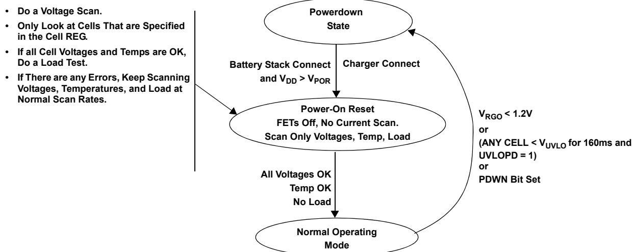
Figure 54. Power-On Reset State Machine
