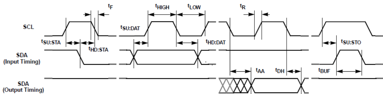
Figure 80. I²C Timing
