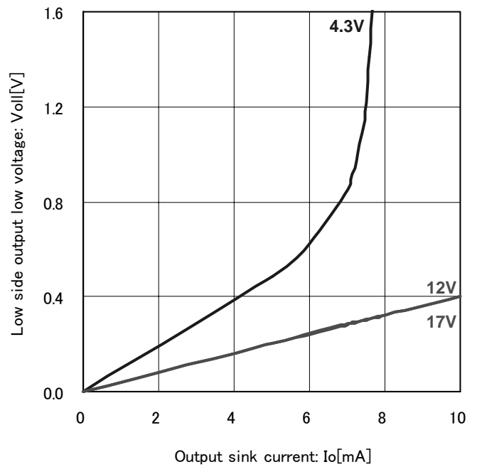
Fig.10 Low side output low voltage (Ta=25°C)
