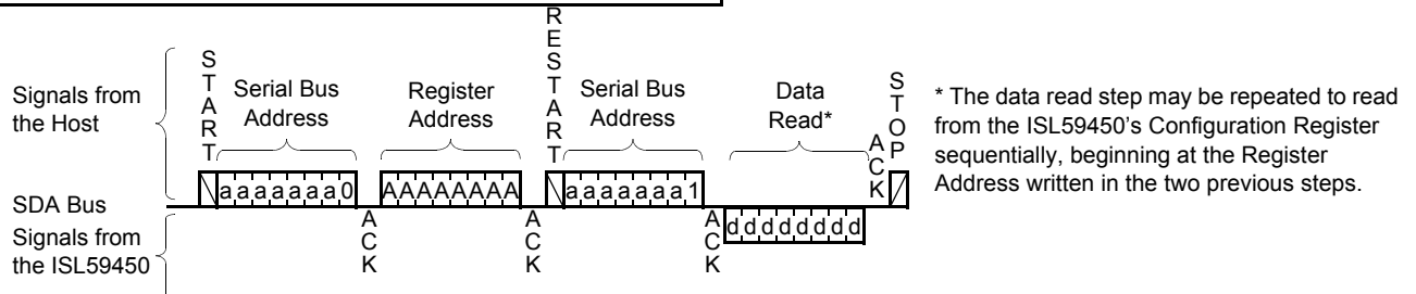
FIGURE 38. CONFIGURATION REGISTER READ
