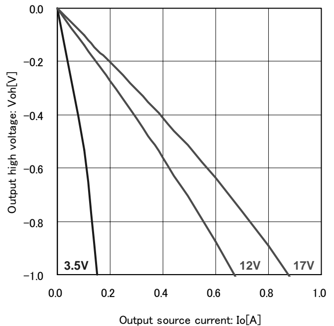
Fig.6 Output high voltage ( T_a=25^\circ\text{C} )
