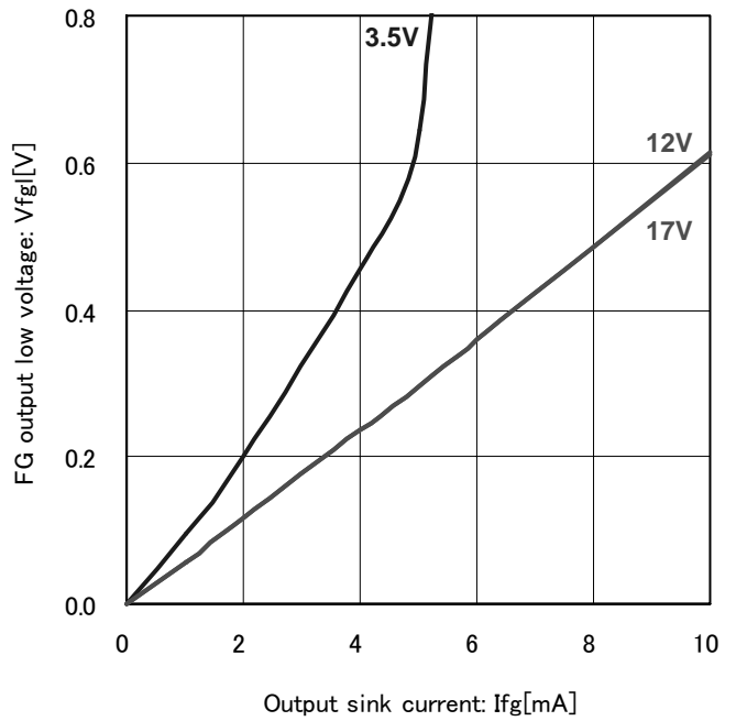
Fig.12 FG output low voltage (T a =25°C)
