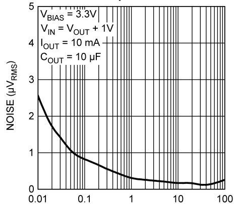
Output Noise
