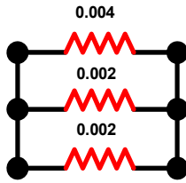
FIGURE 41. INCREASING THE NUMBER OF SHUNT RESISTORS IN PARALLEL TO CREATE A SHUNT RESISTOR VALUE REDUCES THE POWER DISSIPATED BY EACH SHUNT RESISTOR
