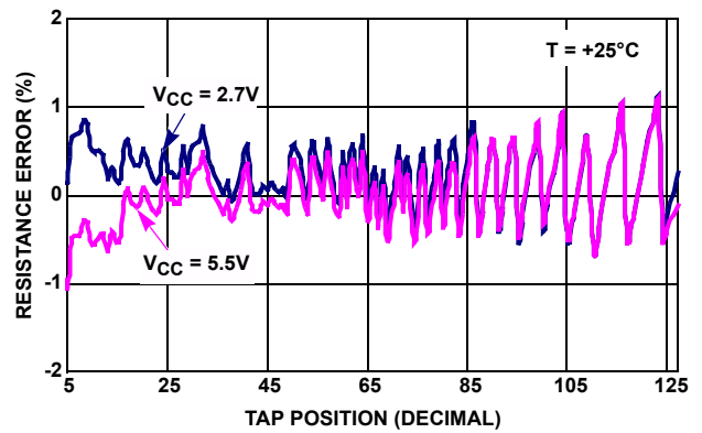
FIGURE 2. RESISTANCE ERROR vs TAP POSITION [I(RW) = V_{CC}/R_{TOTAL}] FOR 10k \Omega (W)
