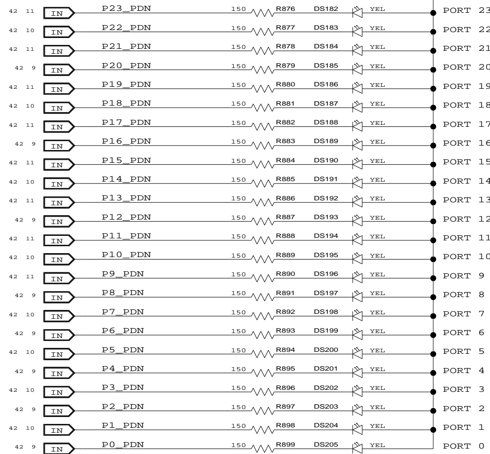
(YELLOW) ACTIVE LOW - PRESENCE DETECT
