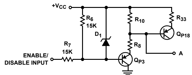
FIGURE 7. SIMPLIFIED SCHEMATIC OF ENABLE/DISABLE FUNCTION
