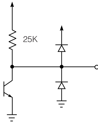
Figure 2-7: Indicator Outputs: HD/ \overline{\text{SD}} , LD
