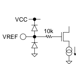
Figure 45. VREF
