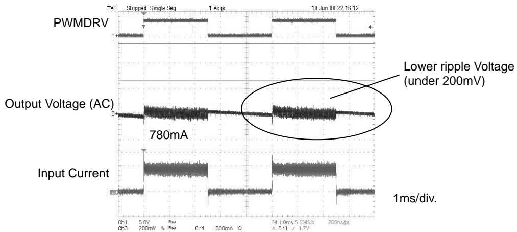
Fig.32 Output voltage ripple for PWM dimming
