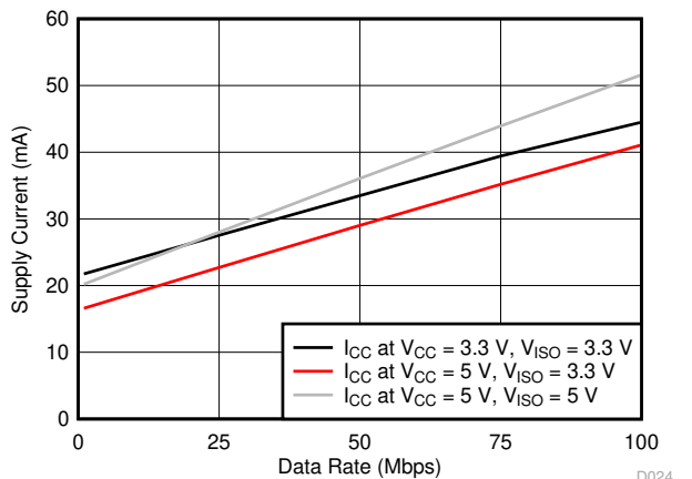
Figure 7-15. ISOW7842 Supply Current vs Data Rate
