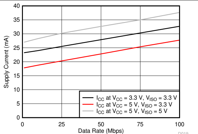
Figure 7-18. ISOW7843 Supply Current vs Data Rate
