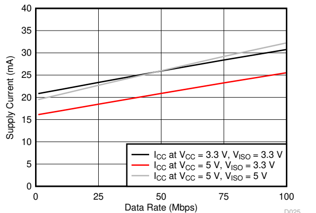
Figure 7-16. ISOW7842 Supply Current vs Data Rate
