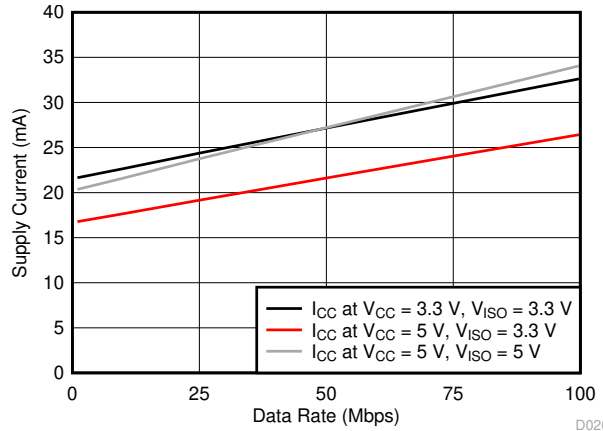
Figure 7-16. ISOW7842 Supply Current vs Data Rate
