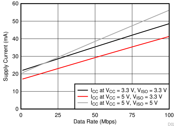
Figure 7-15. ISOW7842 Supply Current vs Data Rate
