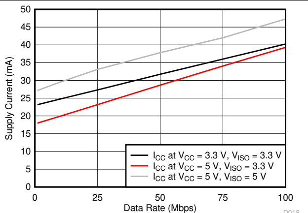
Figure 7-17. ISOW7843 Supply Current vs Data Rate
