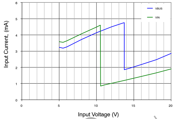
Figure 14. Quiescent Current vs. Input Voltage, I_{SYS} = 0\text{ A} , No Battery, LDO Off, NTC = GND, V_{BUSOVP} = 13.7\text{ V} , V_{INOVF} = 10.5\text{ V}
