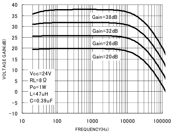
Fig.24 Frequency—Voltage gain
