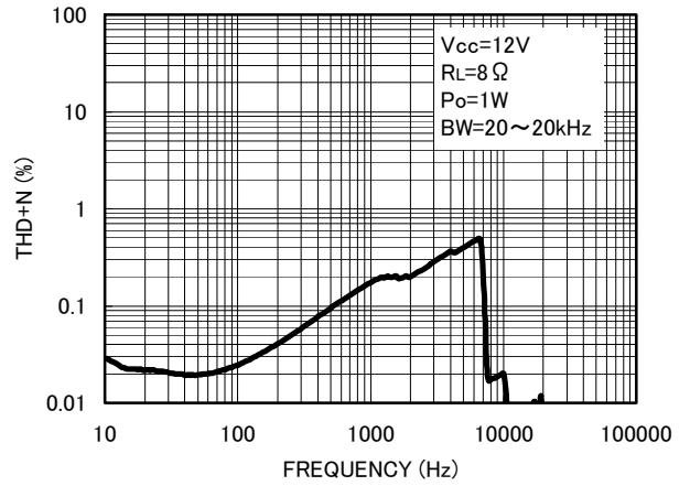
Fig. 2 THD+N – Frequency
