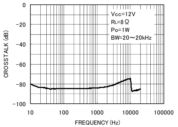
Fig. 4 Crosstalk - Frequency
