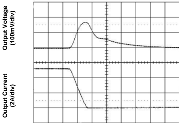
Figure 5. Transient Load Response (typical Vin, load current steps from 50% to 25% at a slew rate 0.1A/µs)
