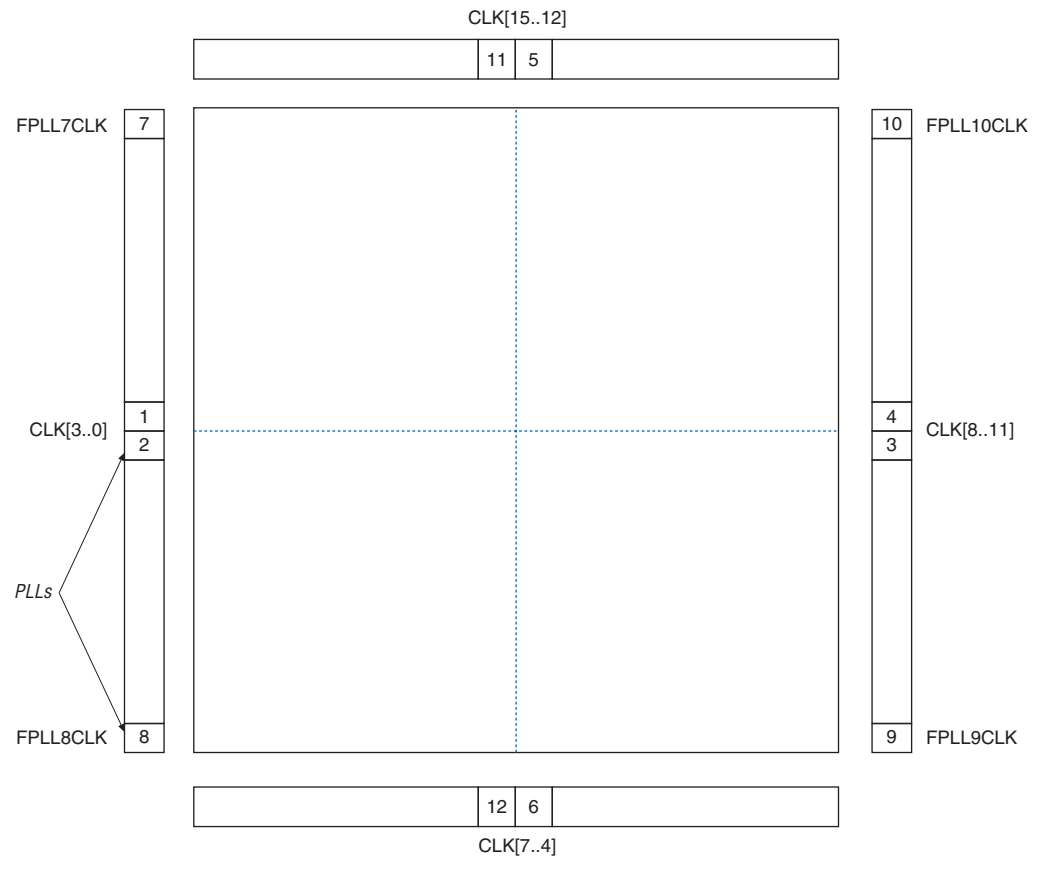
Figure 2–40. PLL Locations
