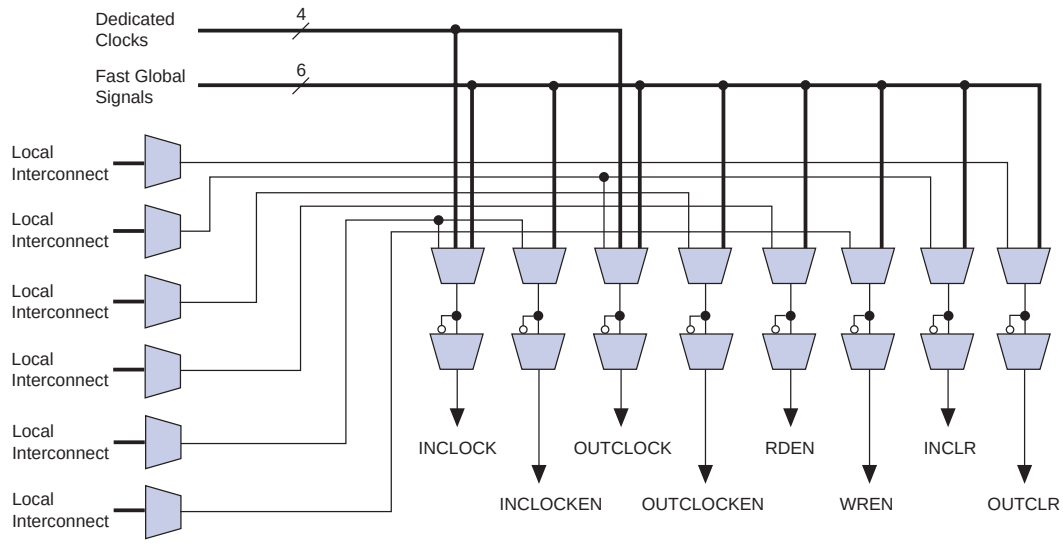
Figure 25. ESB Control Signal Generation
