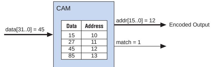
Figure 23. Encoded CAM Address Outputs
