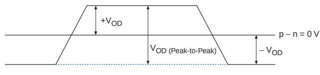
Differential Waveform
