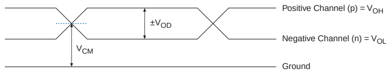
Single-Ended Waveform
