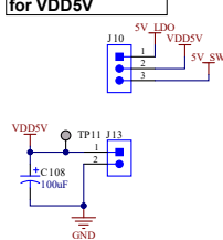
Figure 15-5. DS90UB954-Q1EVM Power Distribution Circuits - Page 4
