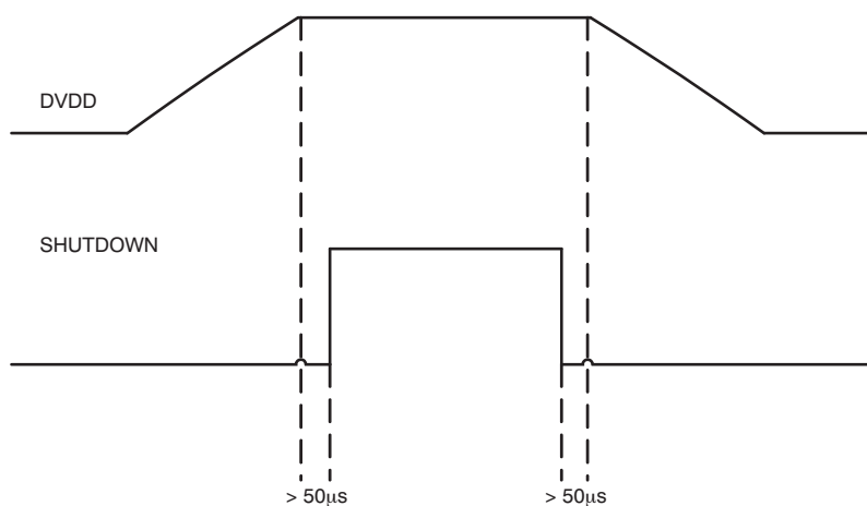
Figure 4. Recommended Power-Up/-Down Sequence
