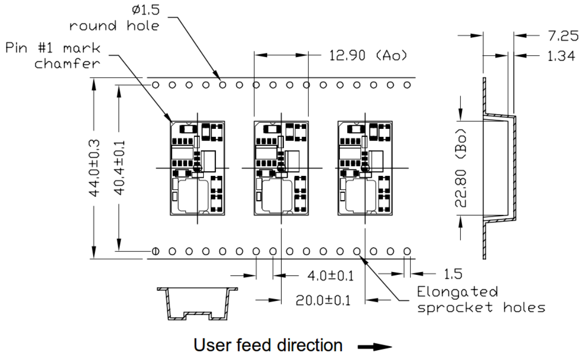
Figure 53. Tape and Reel
