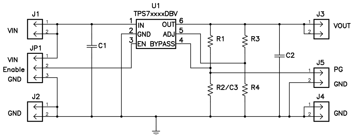
Figure 4. DEM-SOT23LDO Schematic
