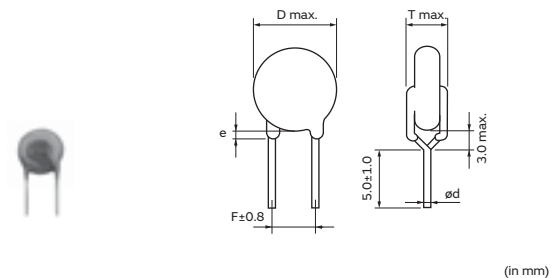
[Bulk] Vertical Crimp Short (B3)
