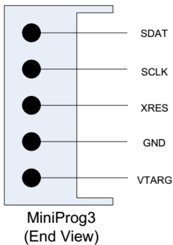
Figure A-5. Pinout for MiniProg3
