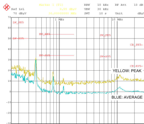
LMS3655-Q1 Conducted EMI: V_{\text{OUT}} = 5\text{ V} , I_{\text{OUT}} = 5\text{ A}
