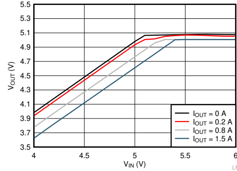
Figure 6-8. Dropout Curve
