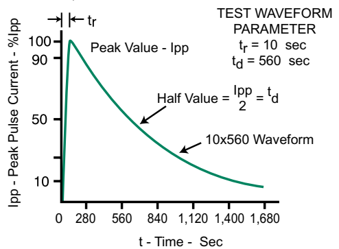
10x560μS PULSE WAVE FORM
