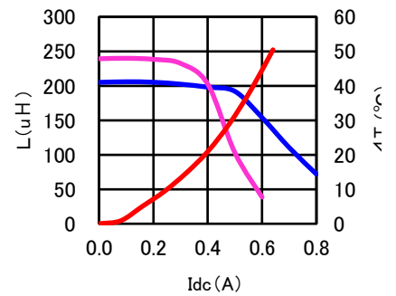
CDRH60D45BT150NP-221MC
