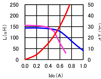
CDRH60D45BT150NP-151MC
