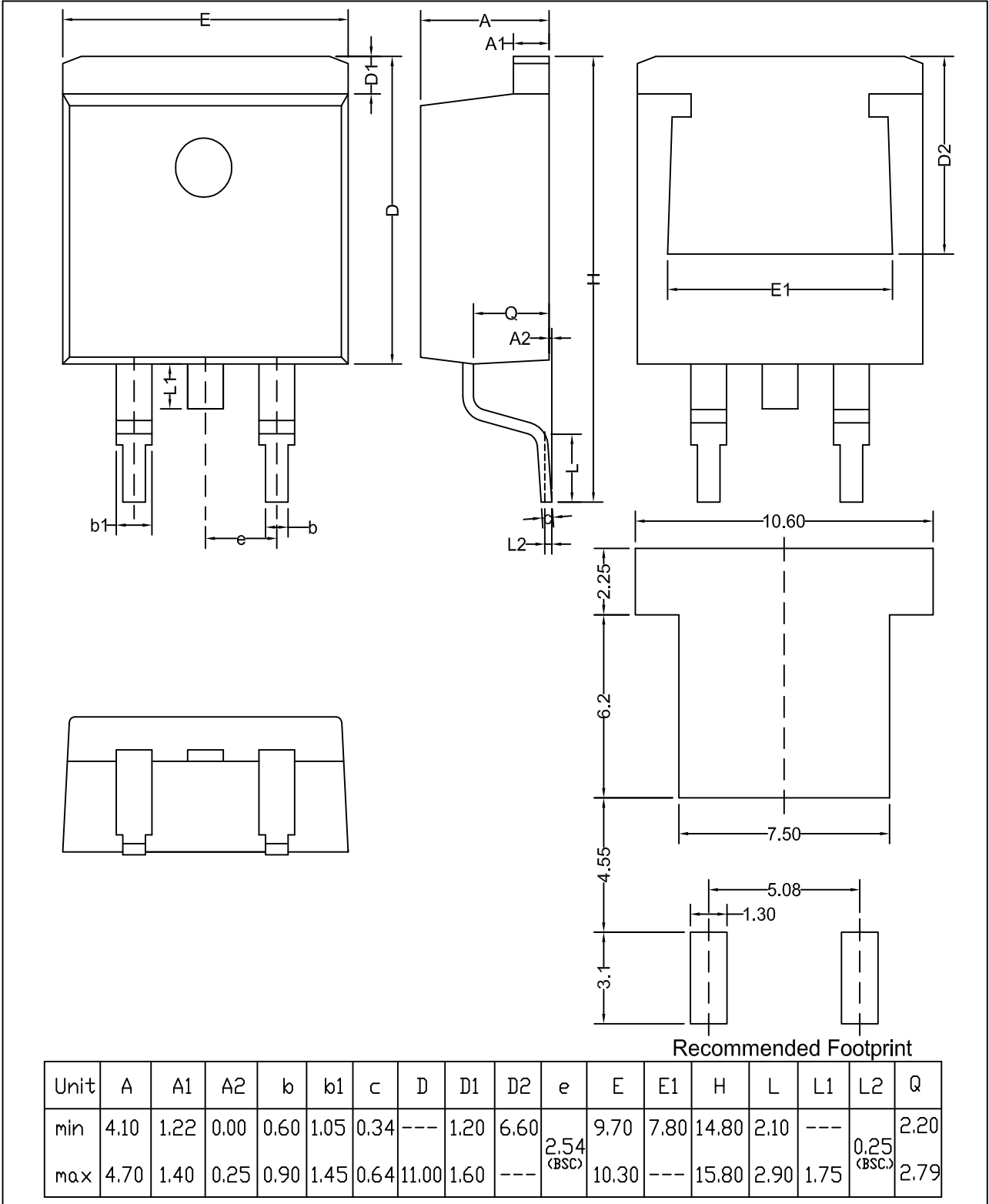
Fig. 8. Package outline TO263
