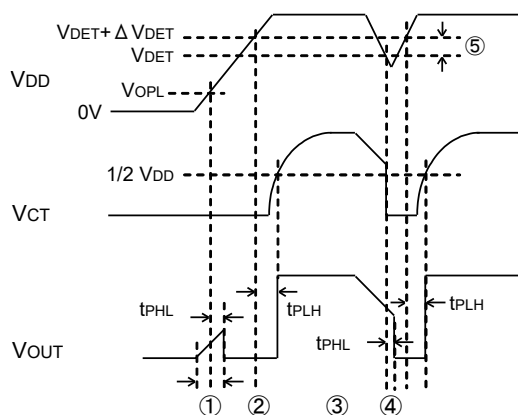
Fig.17 Timing Waveforms
