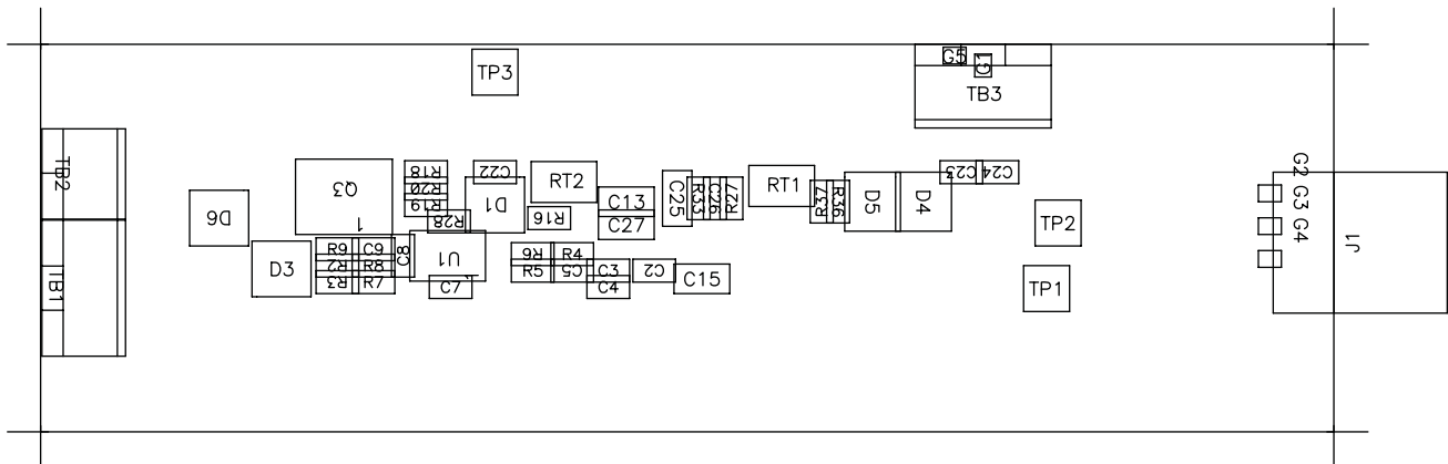
Figure 2. Top Assembly
