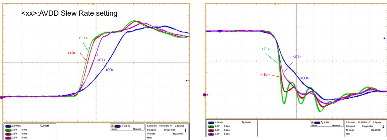
Figure 79. AVDD Switching Slew Rate (VIN=3.3V, AVDD=10.5V, Freq=2.1MHz, L=4.7µH, IAVDD=100mA)
