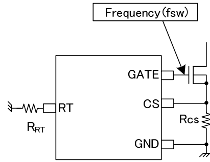
Figure 21. RT terminal setting example
