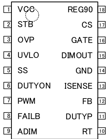
Figure 3. Pin Configuration
