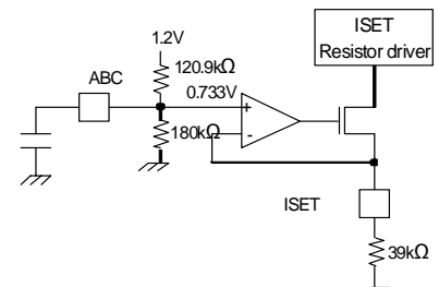
Figure 47. PWM dimming application
