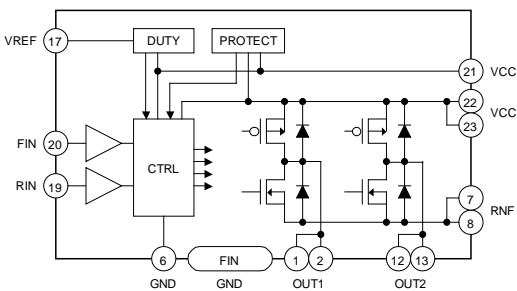
Figure 5. BD6232FP
