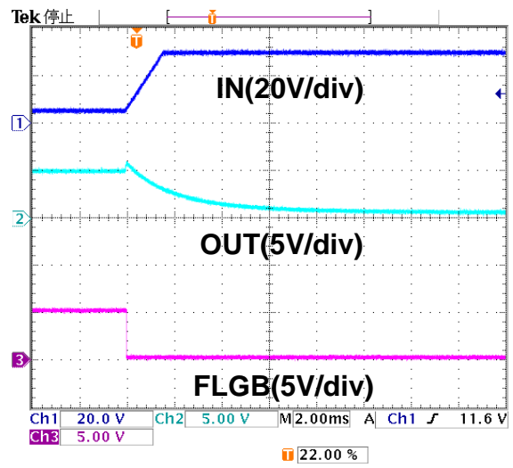
Figure 4. Input Steps (5→30V)
