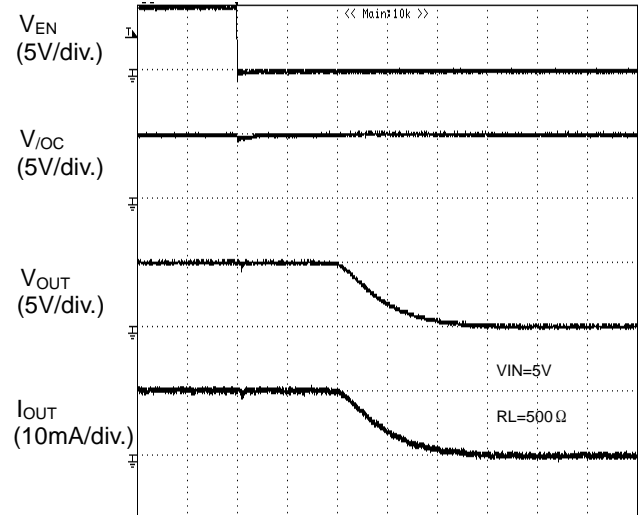
TIME (1us/div.) Figure 55. Output Fall Characteristic
