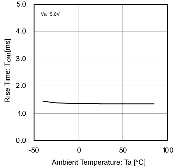
Figure 35. Output Rise Time vs Ambient Temperature
