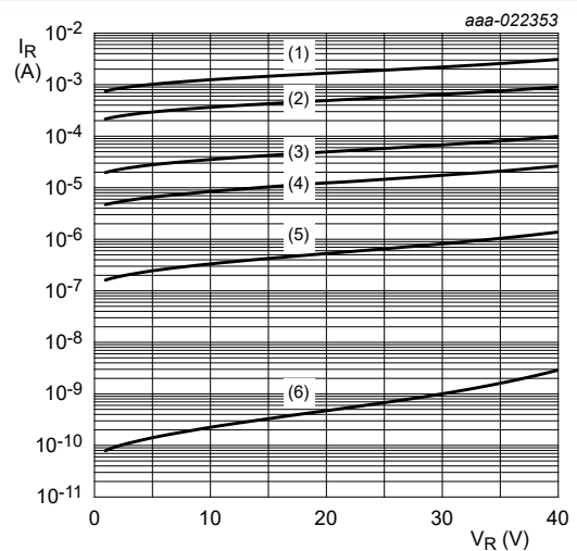
pulsed condition (1) T_j = 150 \text{ }^\circ\text{C} (2) T_j = 125 \text{ }^\circ\text{C} (3) T_j = 85 \text{ }^\circ\text{C} (4) T_j = 65 \text{ }^\circ\text{C} (5) T_j = 25 \text{ }^\circ\text{C} (6) T_j = -40 \text{ }^\circ\text{C}
