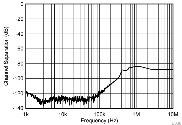
Figure 6-31. Channel Separation
