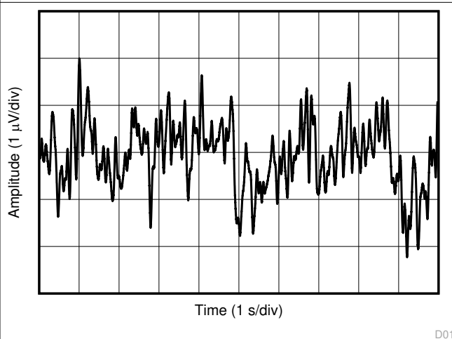
Figure 6-12. 0.1 Hz to 10 Hz Integrated Voltage Noise
