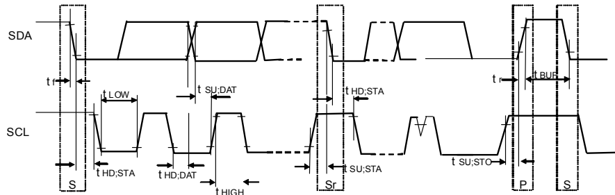
Fig.14 I 2 C BUS Interface Timing
