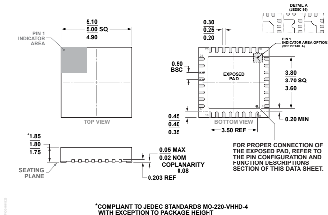
Figure 26. 32-Lead Lead Frame Chip Scale Package [LFCSP] 5 mm × 5 mm Body and 1.8 mm Package Height (CP-32-26) Dimensions shown in millimeters
