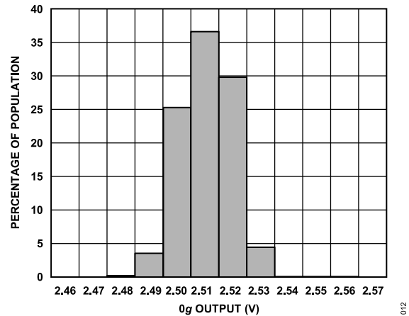
Figure 21. ADXL1001/ADXL1002 0 g Output Population
