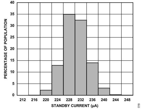
Figure 19. ADXL1001/ADXL1002 Standby Current Histogram at 5 V
