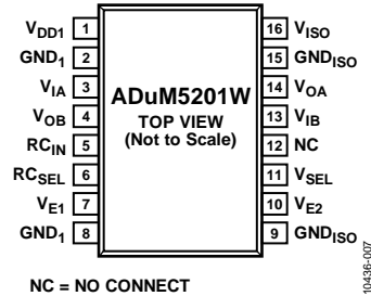
Figure 7. ADuM5201W Pin Configuration
