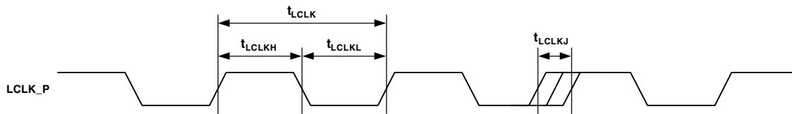
Figure 9. Reference Clocks—Local Clock (LCLK) Cycle Time
