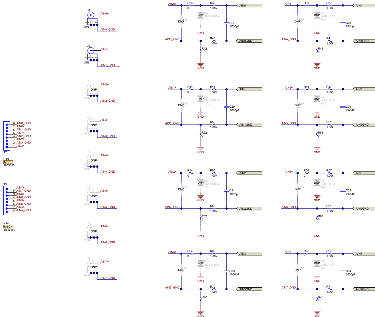
Figure 27. ADS8686SEVM-PDK Schematic
